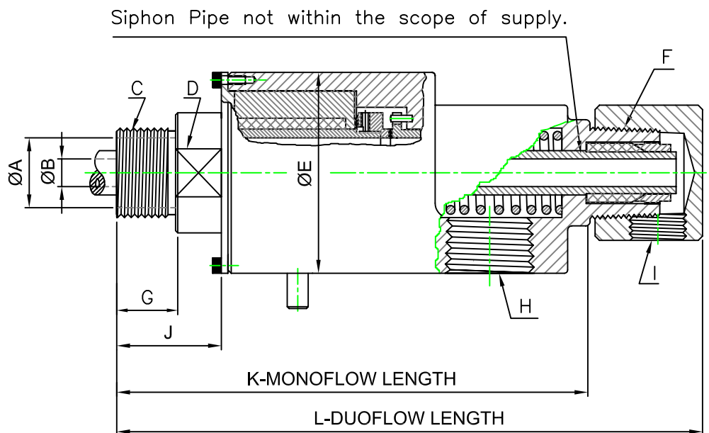
MOUNTING ARRANGEMENT
