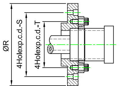
MOUNTING ARRANGEMENT
