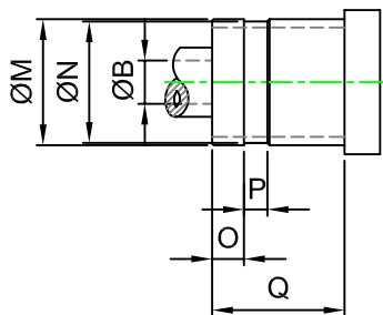
QUICK CONNECTION ROTOR DETAIL
